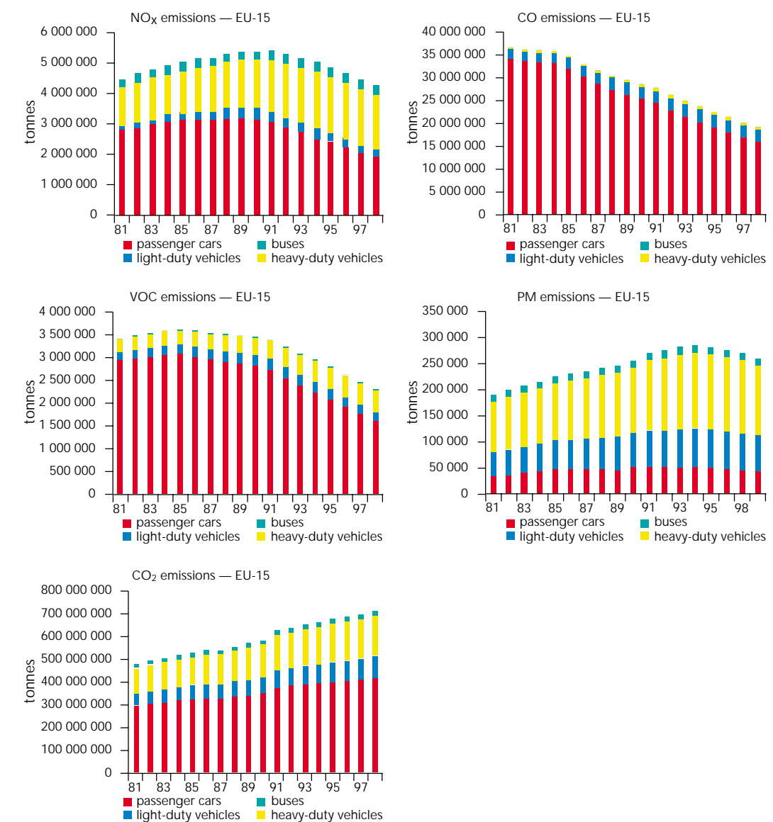
Total NO x , CO, exhaust VOC, PM and CO 2 central emission estimates and contribution of different vehicle categories for the period 1981-98
