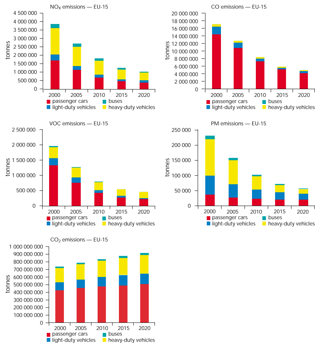
Figure 4. NO x , CO, exhaust VOC, PM and CO 2 emission trends and contribution of different vehicle categories for the period 2000–20
