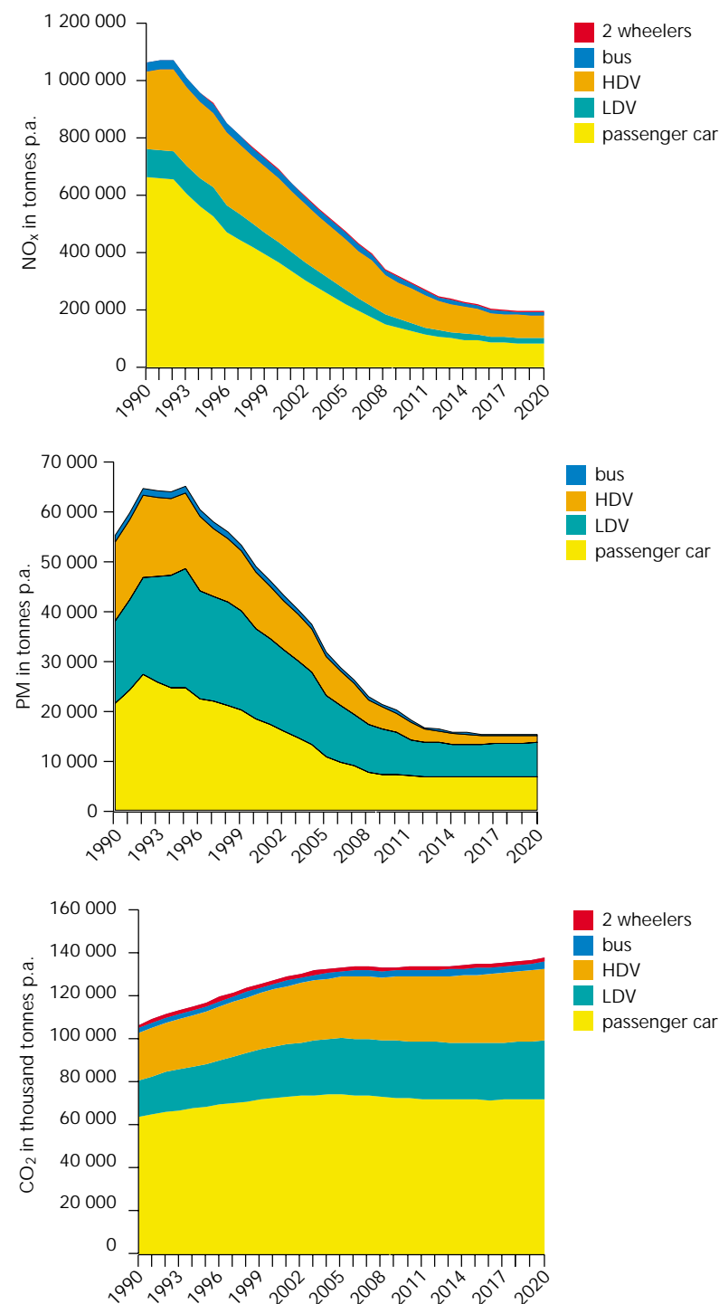
Figure A5. Development of \text{NO}_x , PM and \text{CO}_2 emissions from transport in France 1990–99 and projections to 2020
