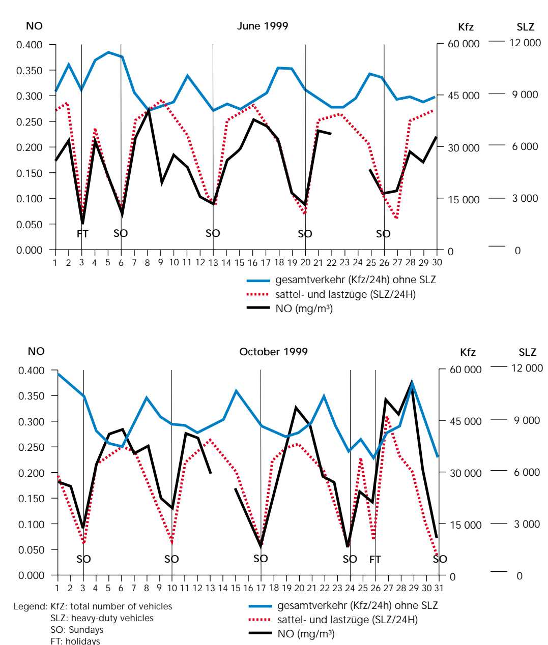
Time series of NO concentration at Vomp (A12 motorway) in June and October 1999 correlated with the traffic volumes (total vehicles and HDVs)
