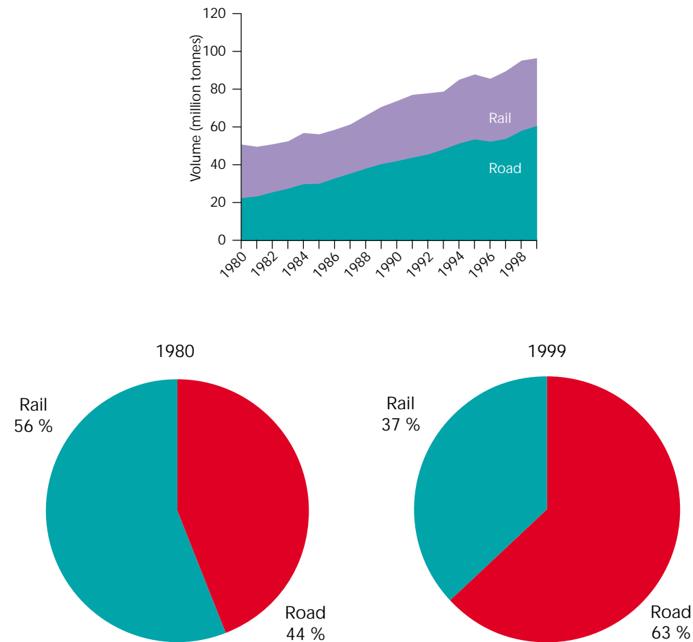
Figure A1. Development of transalpine freight transport (Mont Cénis-Brenner) 1980-99
