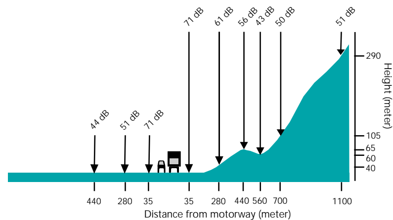
Figure 12. Noise spread in mountainous areas compared with lowland areas
