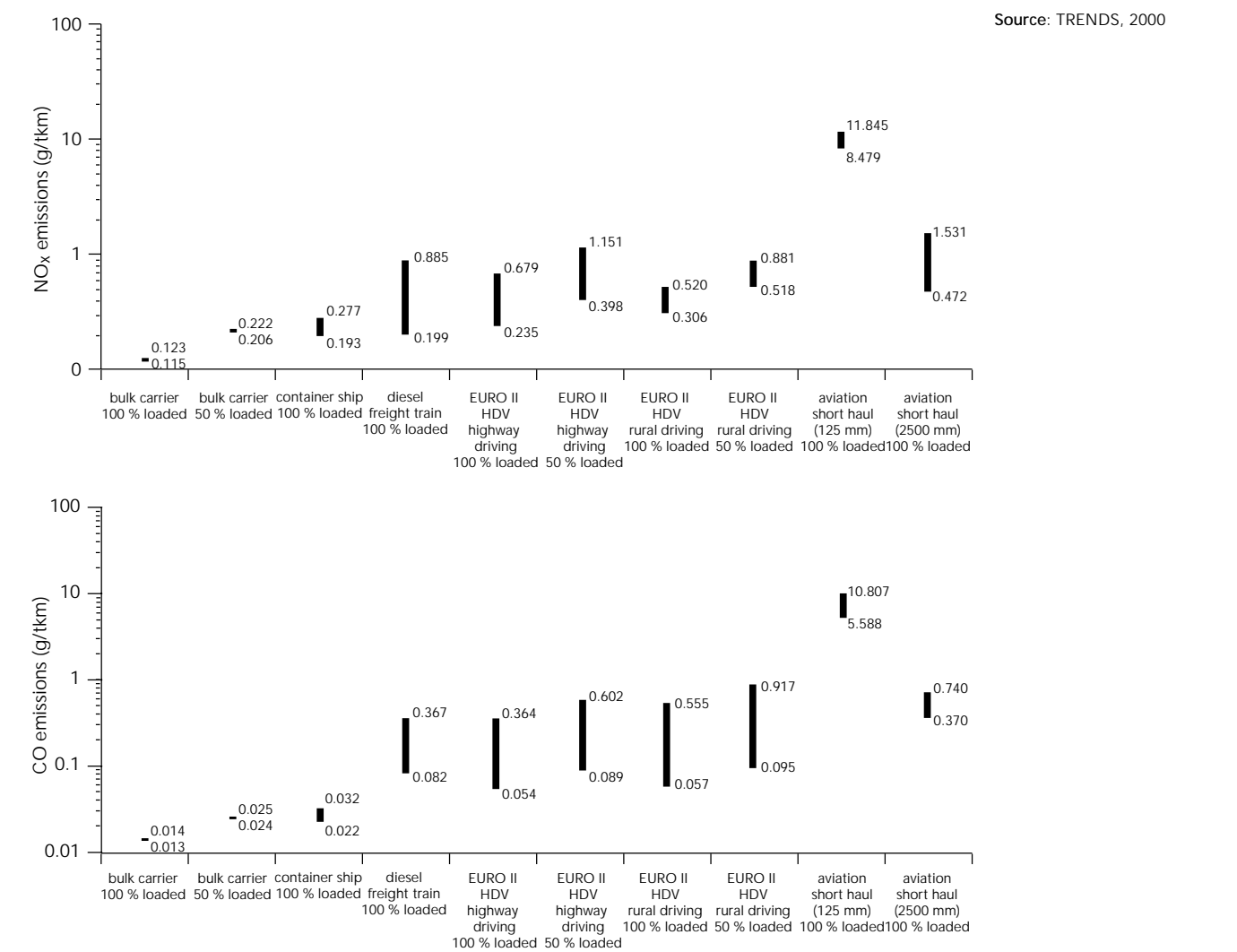
NO x and CO emission estimates per freight tonne-km for different modes of freight transport
