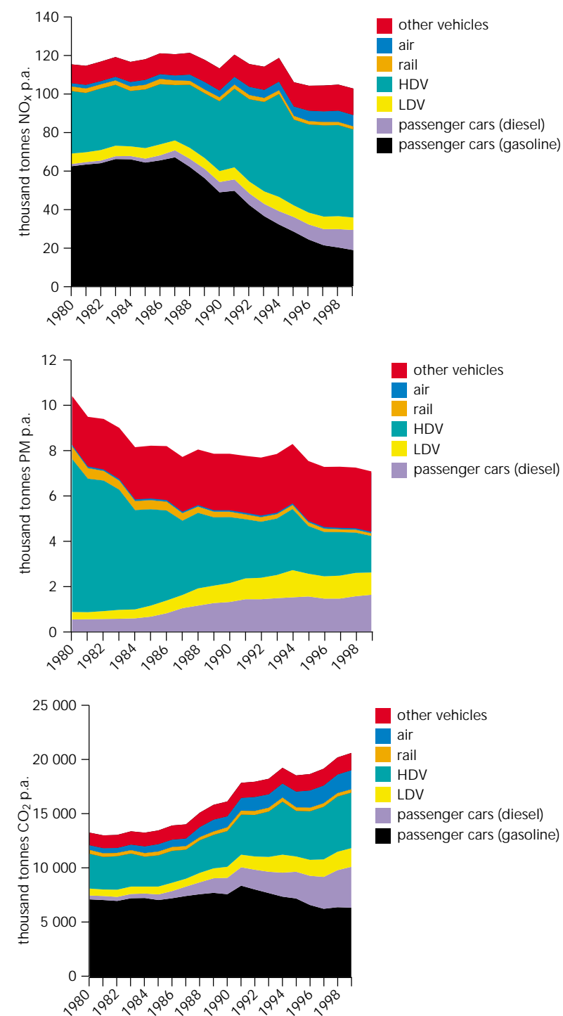
Development of NO x , PM and CO 2 emissions from transport in Austria 1980-99 Figure A4.
