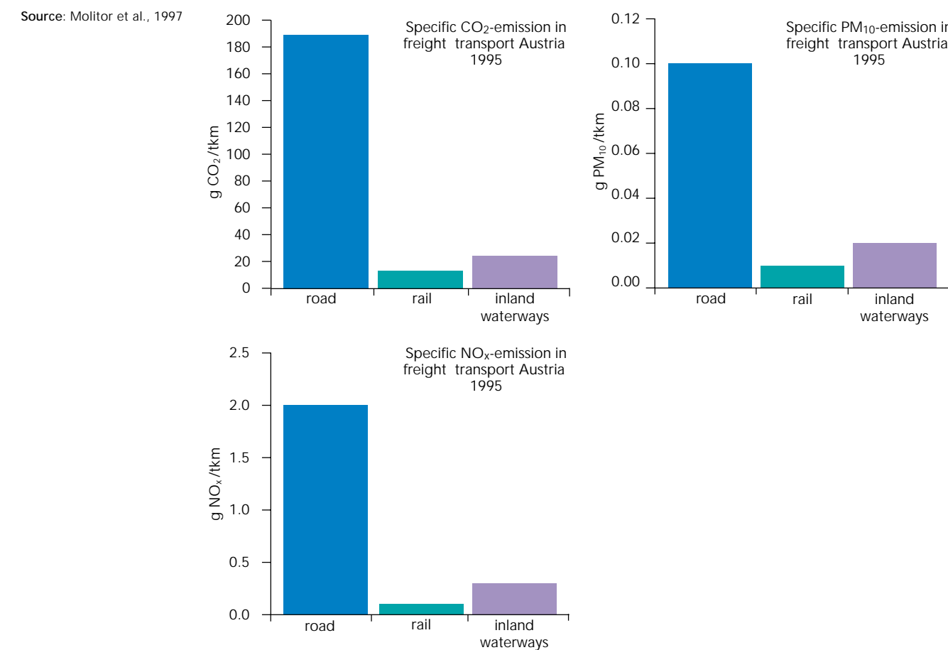
Figure 6. Specific emissions of air pollutants and CO 2 from different transport modes of freight transport — Austria, 1995
