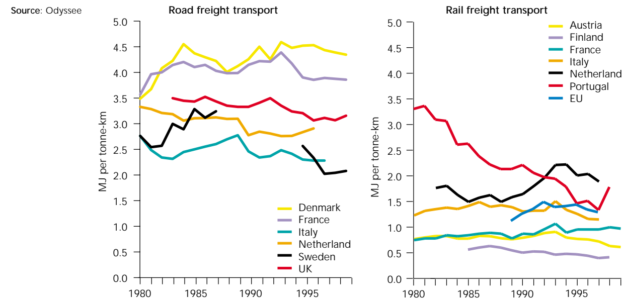
Figure 5. Energy use per tonne-km of road and rail freight transport — selected EU countries
