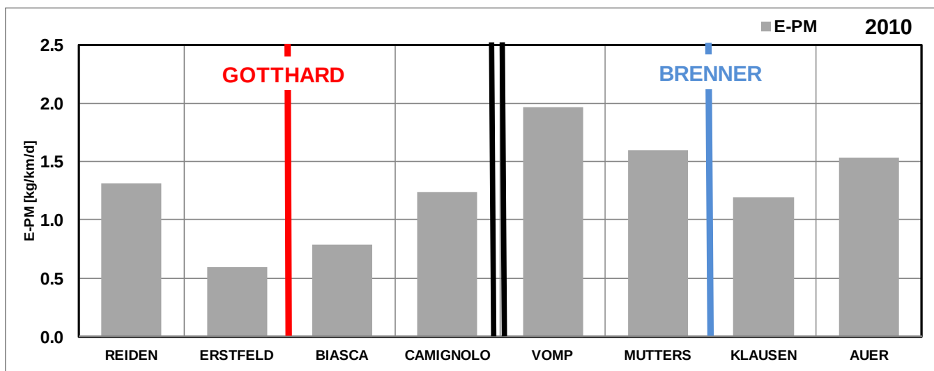
Figure 5.1: Emissions of NO x , NO 2 and PM at Gotthard and Brenner in 2010.
