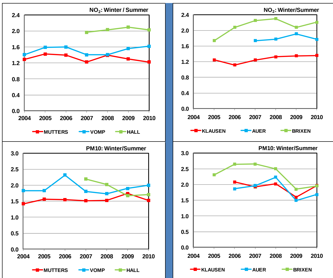
Figure 3.7: Seasonal variation of NO x , NO 2 and PM 10 between winter and summer at Brenner, 2004-2010.
