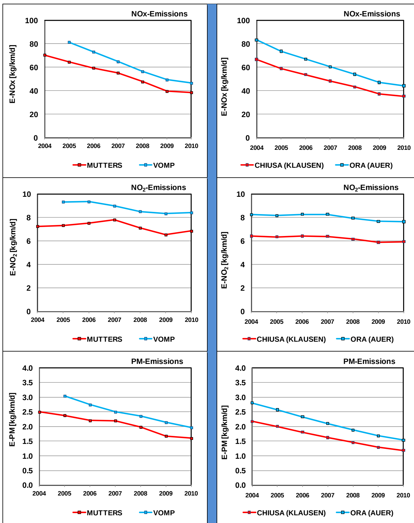
Figure 5.5: Emissions of NO x , NO 2 and PM at Brenner, 2004-2010.
