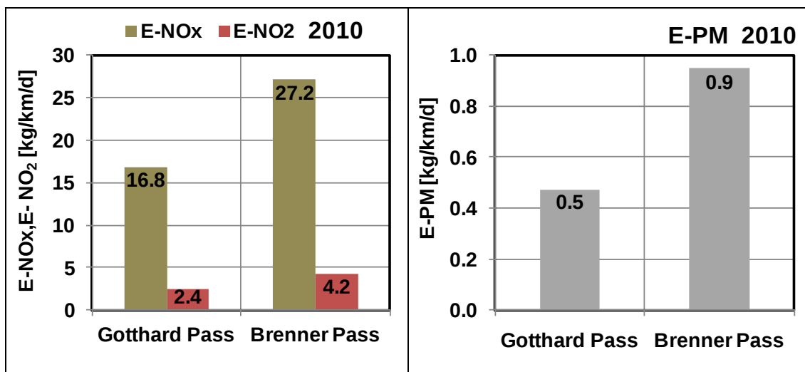
Figure 5.2: Emissions of NO x , NO 2 and PM at Gotthard and Brenner-Passes in 2010.
