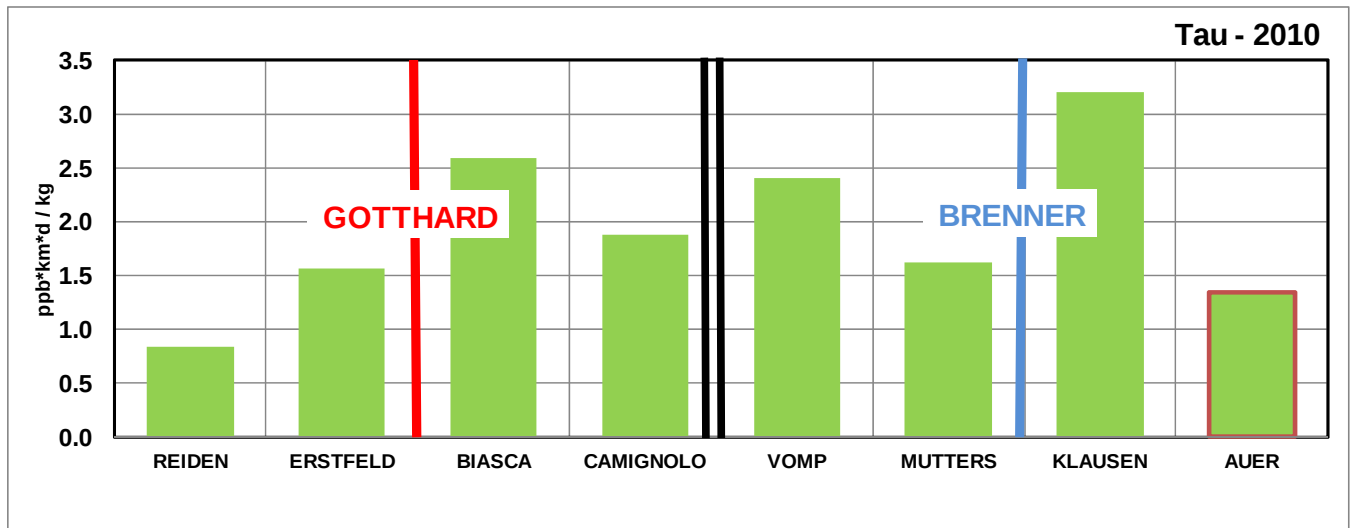
Figure 6.3: Tau: Ration of NOx air concentration / NOx-Emission at Gotthard and Brenner in 2010.
