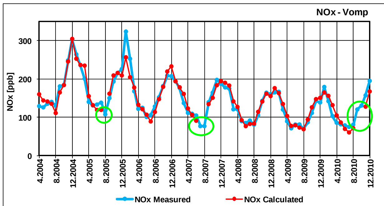
Figure 8.1: Monthly average of NO x for Vomp (Tyrol), April 2004 - Dec 2010.
