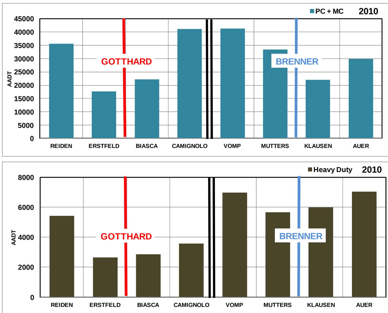
Figure 4.3: AADT of PC+MC and Heavy Duty categories at Gotthard and Brenner in 2010.
