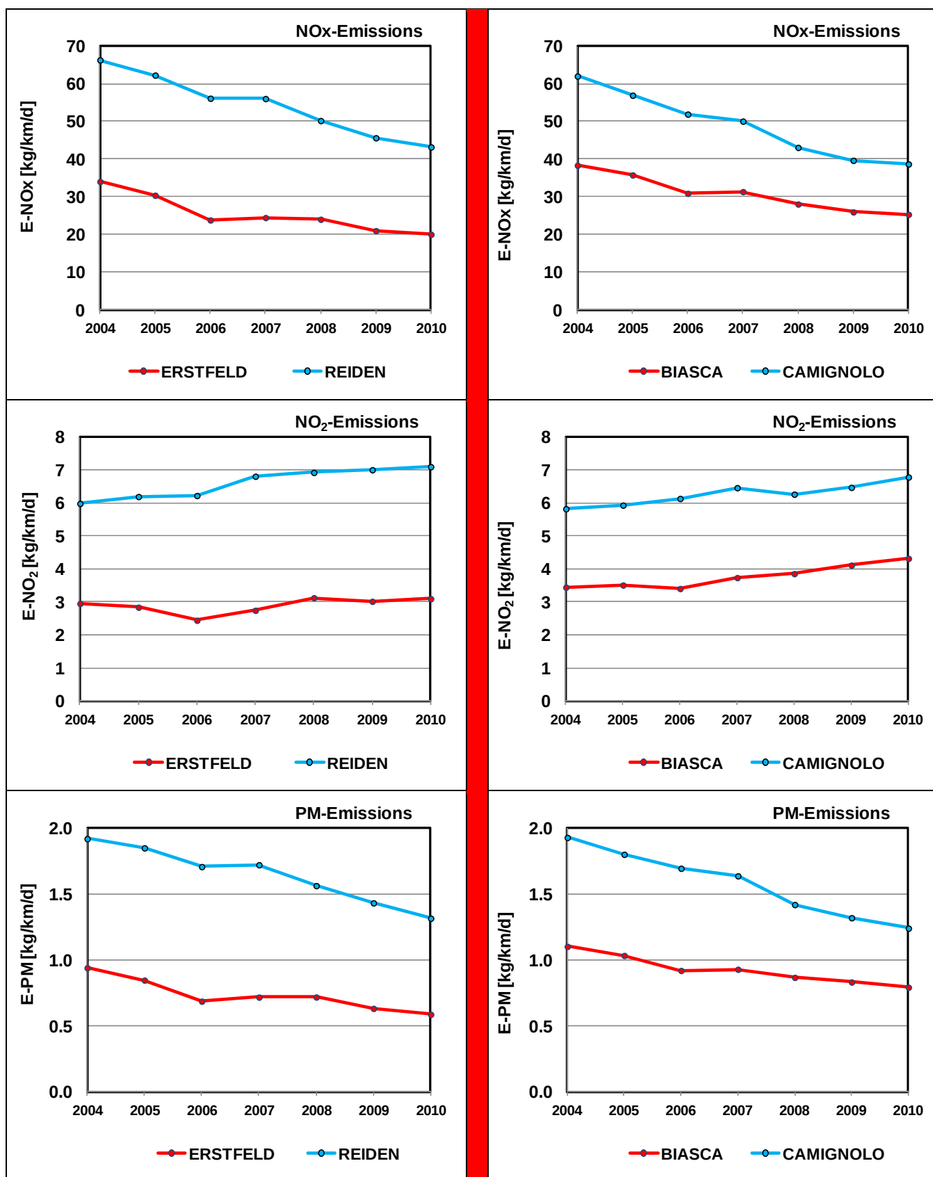
Figure 5.4: Emissions of NO x , NO 2 and PM at Gotthard, 2004-2010.
