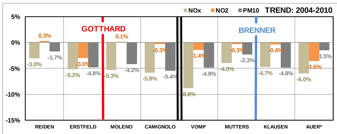
Figure 3.5: Trend (in %) per year for NOx, NO 2 and PM10 at Gotthard and Brenner, 2004 – 2010.
